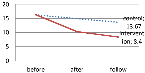
(WCST) Preservation error
