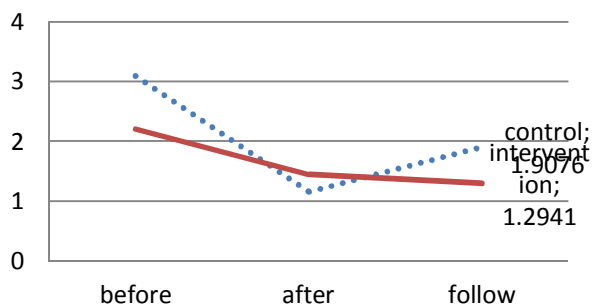
(SCWT) Reaction time
