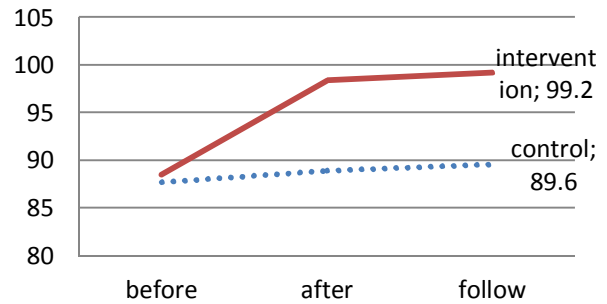
(SCWT) Commission error
