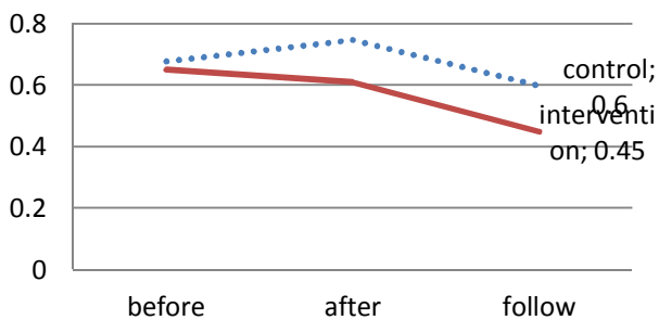
No-Go reaction time
