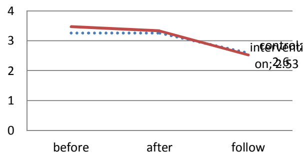
No-go errors
